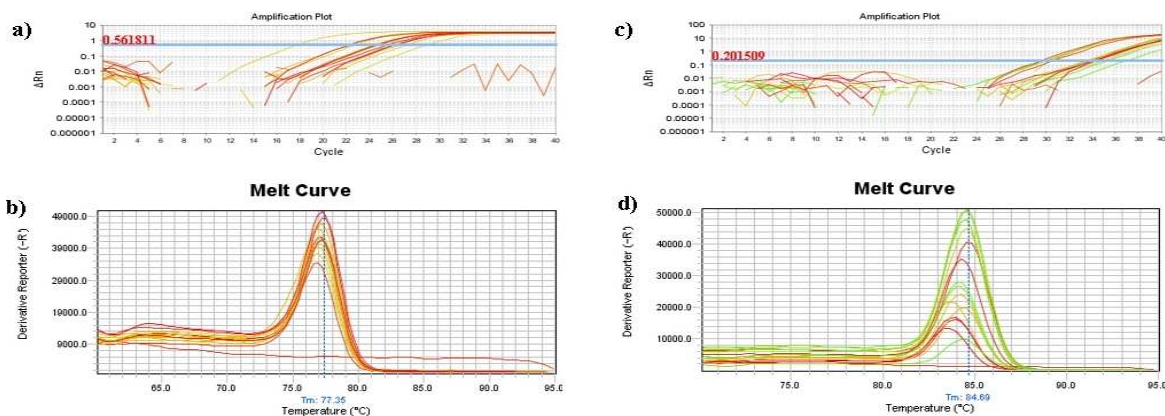
Figure 8: HPRT reference gene amplification in PCR cycles (a) and melting curve (b); Cox-2 gene amplification curve in PCR cycles (c) and its melting curve (d).
