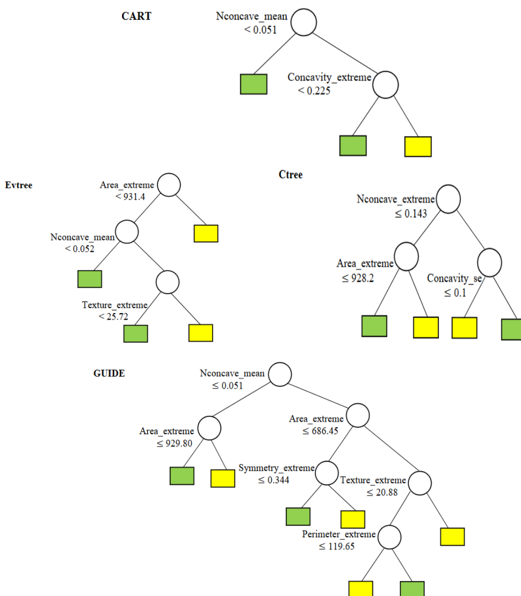
Figure 2. The tree structure of classification tree algorithms (CART, Evtree, Ctree, and GUIDE) for distinguishing between malignant and benign tumors in the Wisconsin Breast Cancer Dataset (Green: benign and yellow: malignant)
